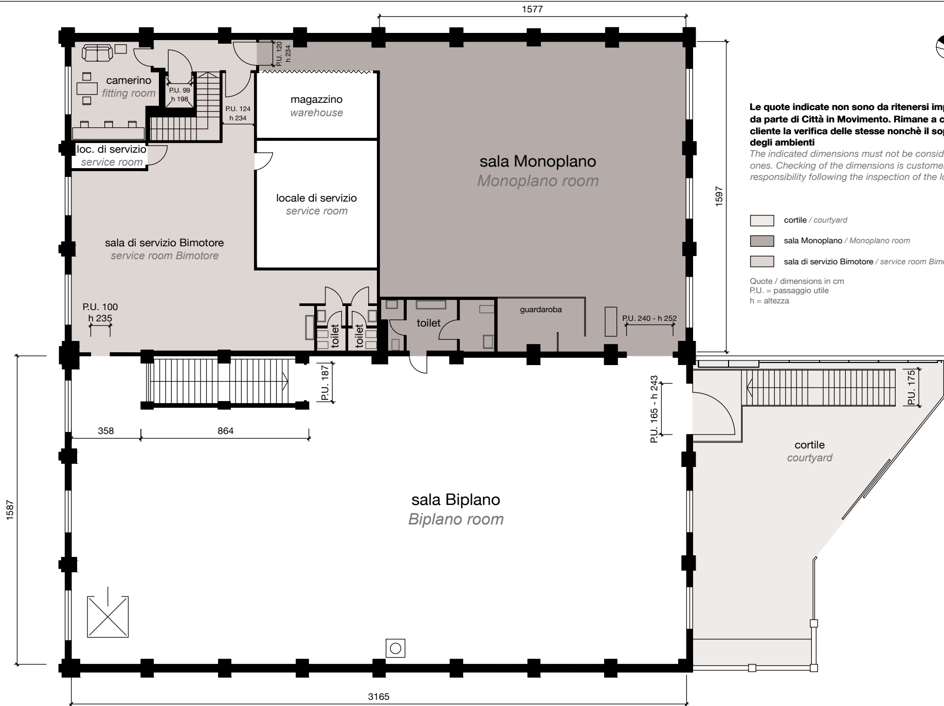
Sala Monoplano / piano primo / first floor plan
